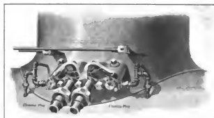
Fig. 3253. Leach Pneumatic Double Sander.
